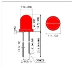
19704261 Diode LED 10MM rouge LED 10MM/R ///
