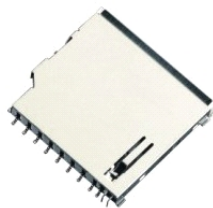
18910017 Support carte SD 11pin 27.6*25*25.5*1.5mm /// HW-SD-001-02
