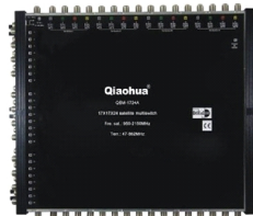
19403011 Multiswitch input 16sat+ant,*17* 24 ports cascadeable Terr.47-862MHz, 5(dB) ,SAT 950-2150MHz /// QSM-1724A/17
